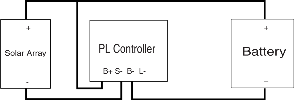
Series Regulation Only.
