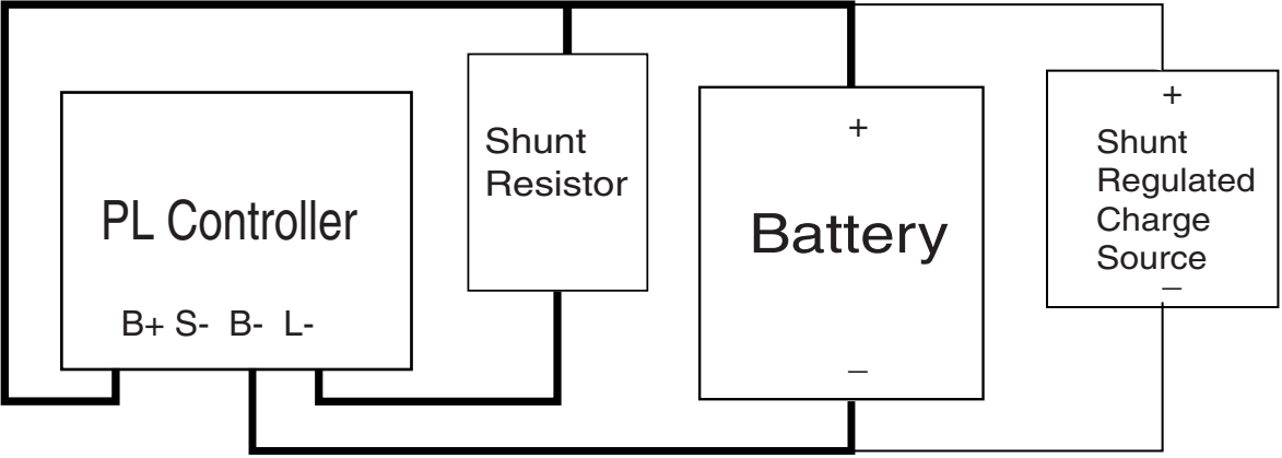
Shunt Regulation Only.
