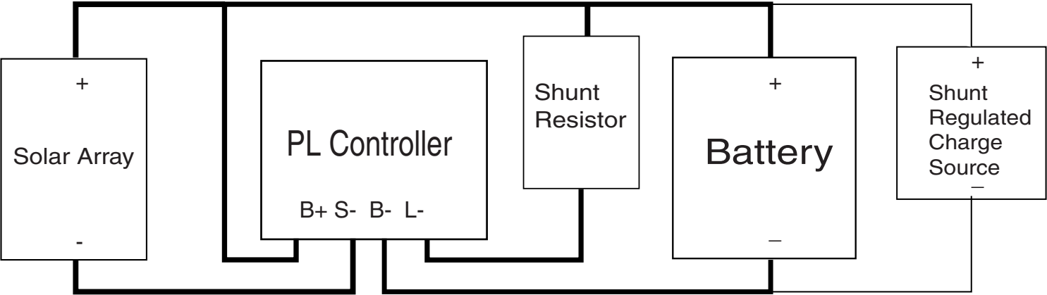
Series and Shunt Regulation Together.
